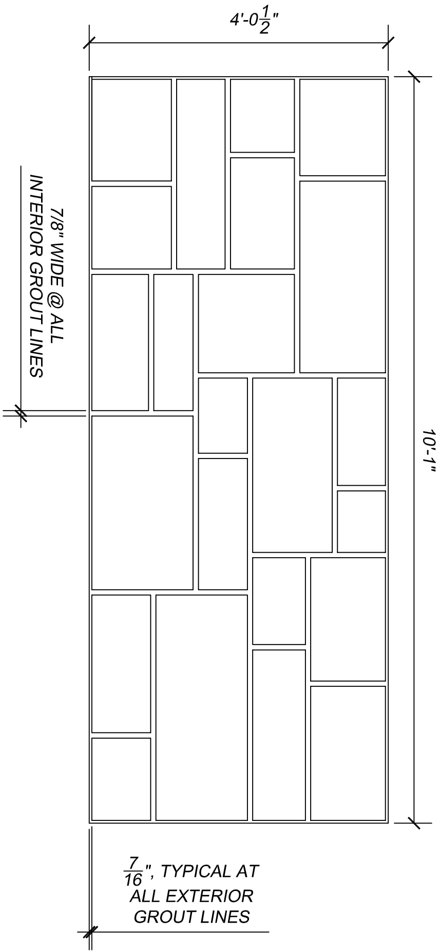
ELEVATION VIEW SCALE: 3/4" = 1'-0"
