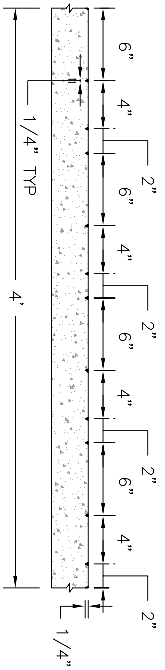
SECTION VIEW
